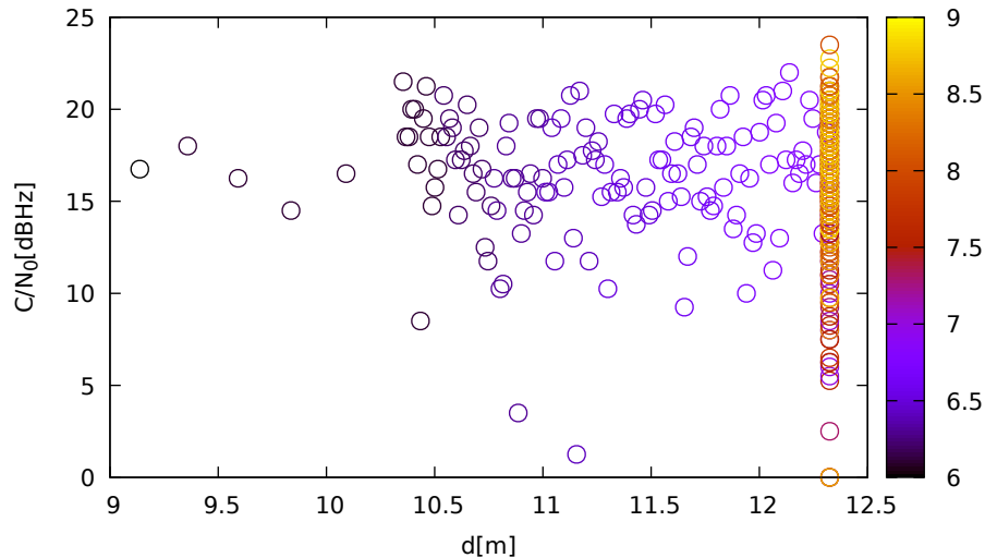
C/N 0 vs distance (JavadLSA at C 3 for G21 at L2)
