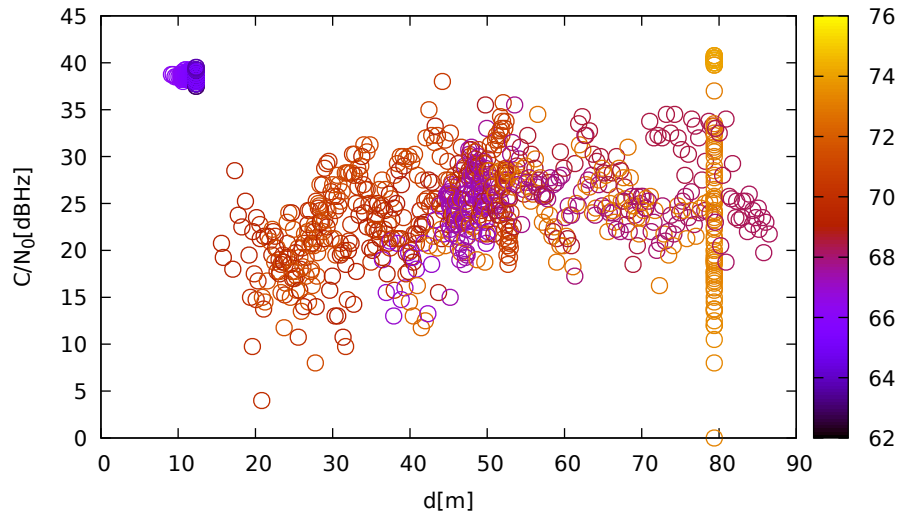
C/N 0 vs distance (JavadLSA at C 3 for G22 at L2)
