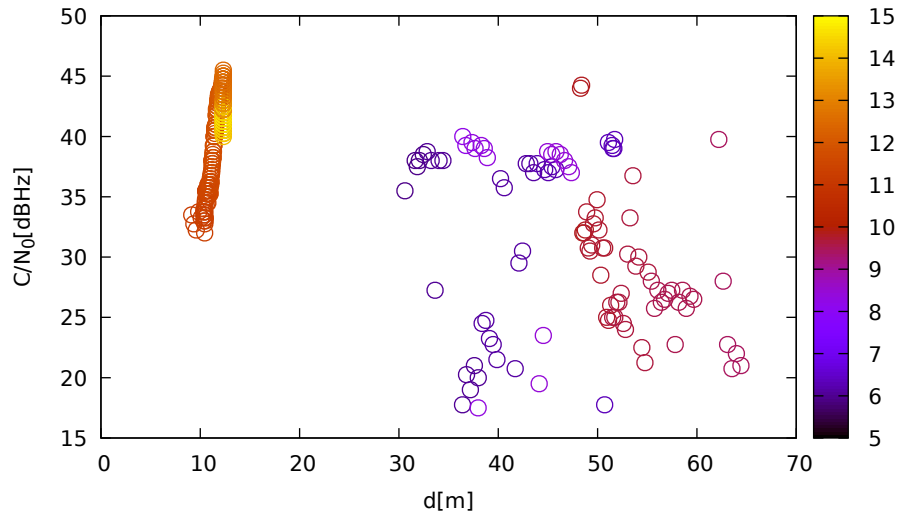
C/N 0 vs distance (JavadLSA at C 3 for G27 at L2)
