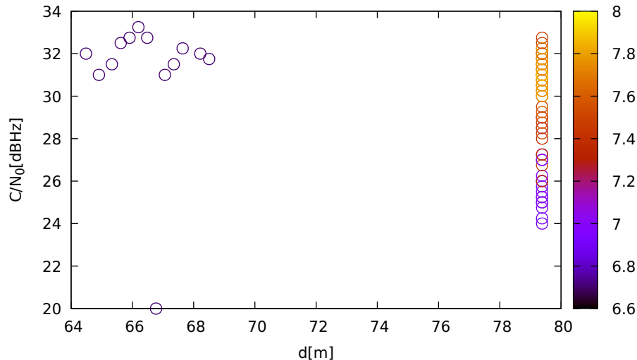
C/N 0 vs distance (JavadLSA at C 3 for G31 at L2)
