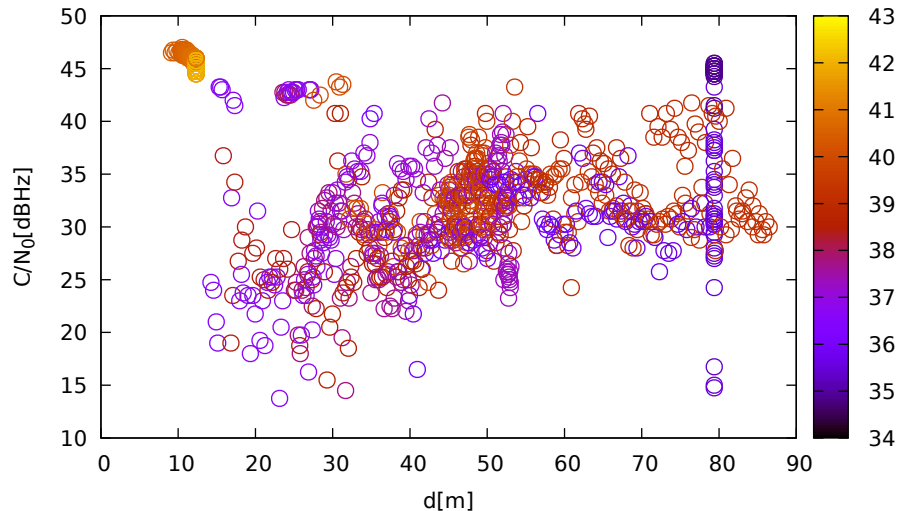
C/N 0 vs distance (JavadLSA at C 3 for G32 at L2)
