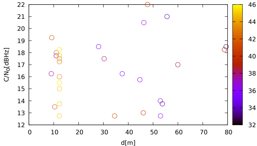
C/N 0 vs distance (JavadLSA at C 3 for R06 at L2)
