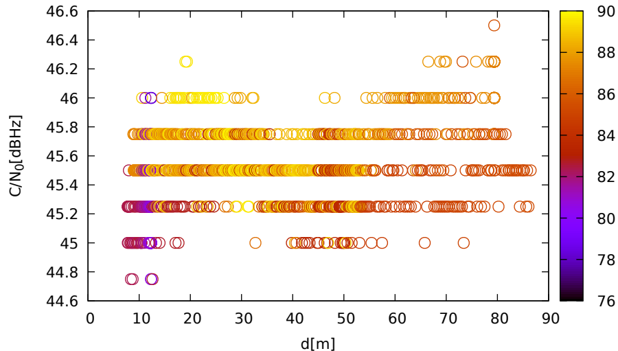
C/N 0 vs distance (JavadLSA at C 3 for R07 at L2)
