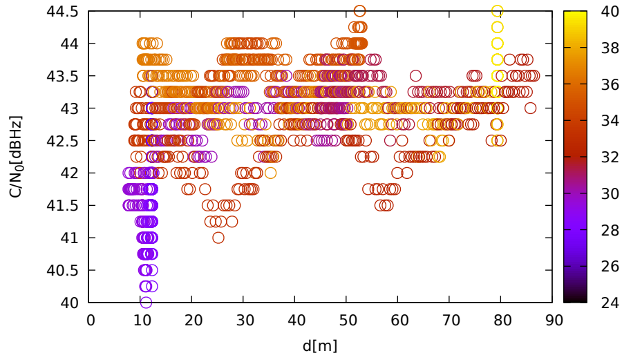
C/N 0 vs distance (JavadLSA at C 3 for R08 at L2)
