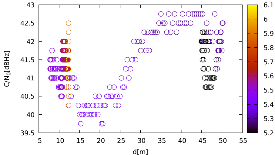
C/N 0 vs distance (JavadLSA at C 3 for R14 at L2)
