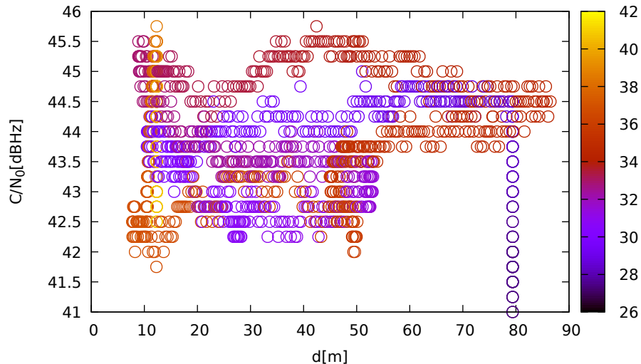
C/N 0 vs distance (JavadLSA at C 3 for R21 at L2)
