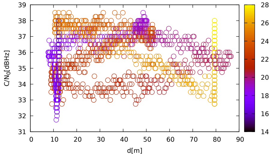
C/N 0 vs distance (JavadLSA at C 3 for R23 at L2)
