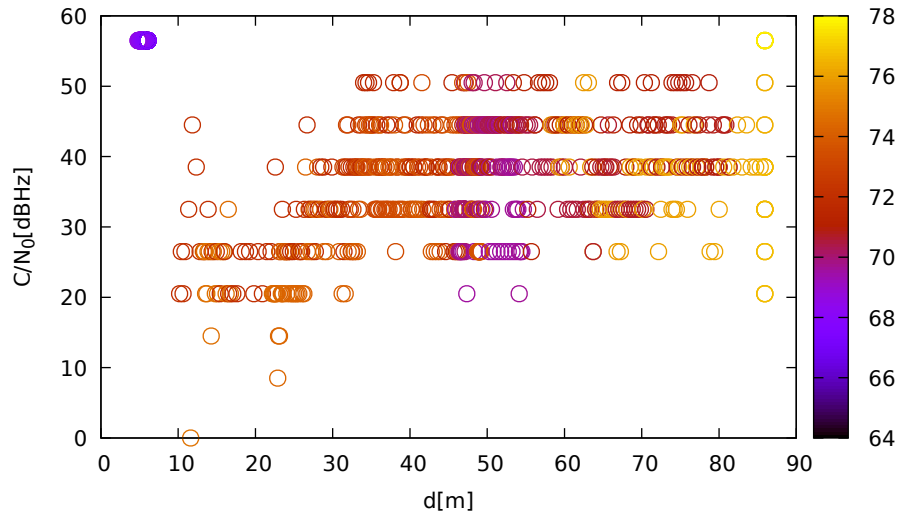
C/N 0 vs distance (LeicaGS15 at C 3 for G01 at L2)
