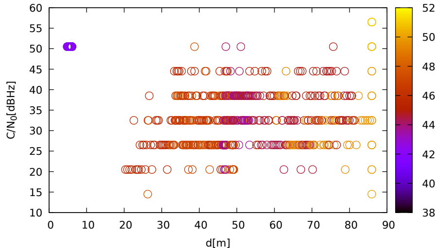
C/N 0 vs distance (LeicaGS15 at C 3 for G03 at L2)
