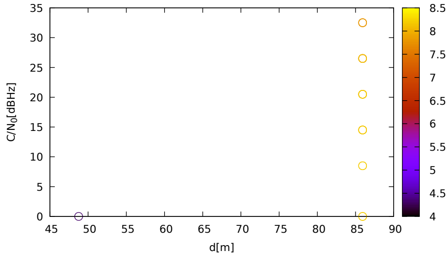
C/N 0 vs distance (LeicaGS15 at C 3 for G04 at L2)
