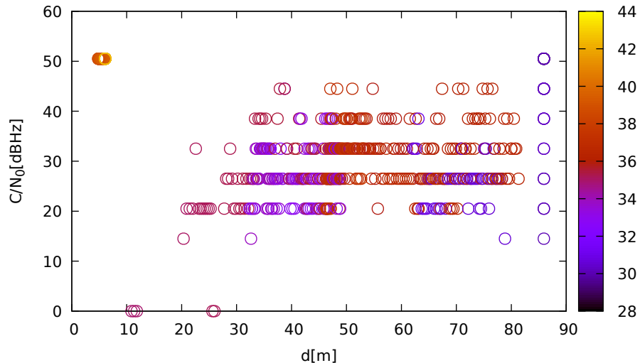
C/N 0 vs distance (LeicaGS15 at C 3 for G08 at L2)
