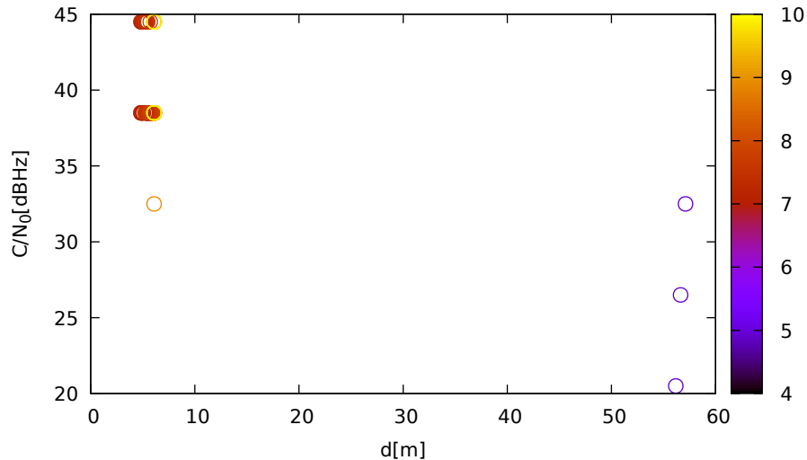
C/N 0 vs distance (LeicaGS15 at C 3 for G10 at L2)
