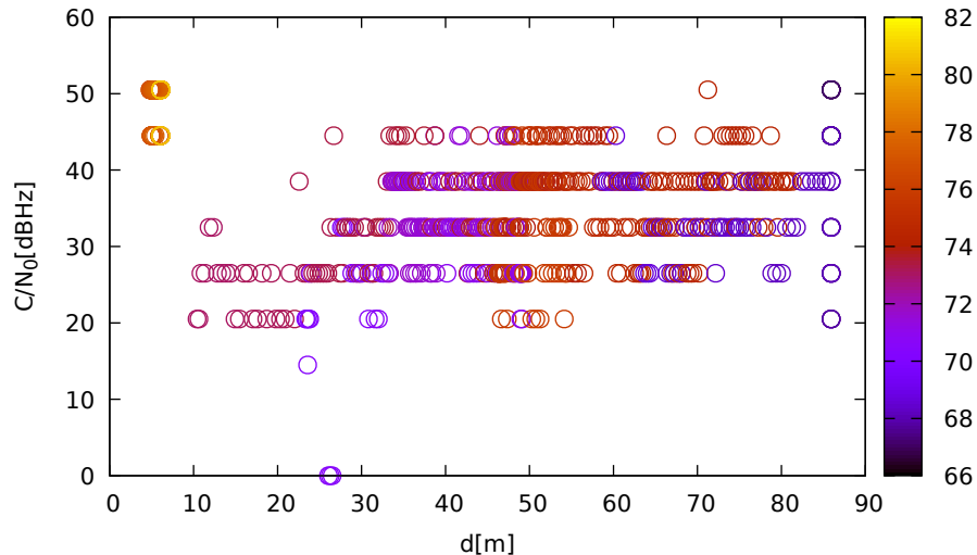
C/N 0 vs distance (LeicaGS15 at C 3 for G11 at L2)
