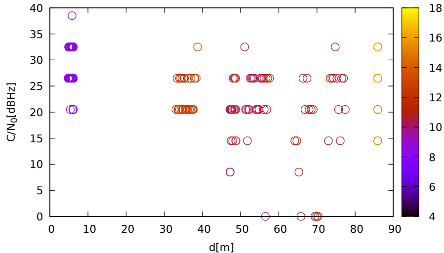
C/N 0 vs distance (LeicaGS15 at C 3 for G17 at L2)
