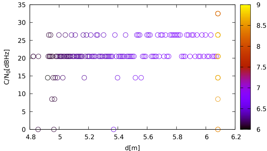
C/N 0 vs distance (LeicaGS15 at C 3 for G21 at L2)
