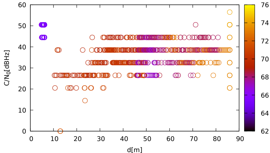
C/N 0 vs distance (LeicaGS15 at C 3 for G22 at L2)
