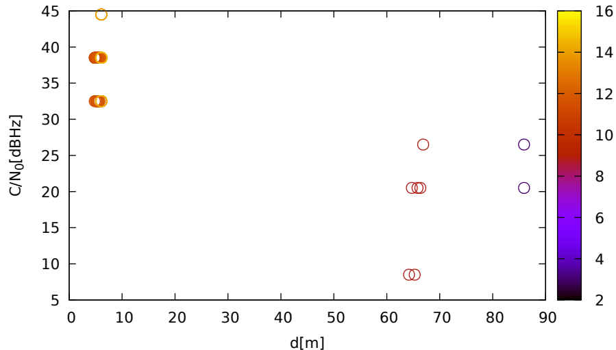
C/N 0 vs distance (LeicaGS15 at C 3 for G27 at L2)
