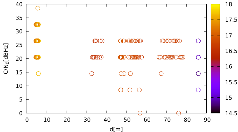
C/N 0 vs distance (LeicaGS15 at C 3 for G28 at L2)
