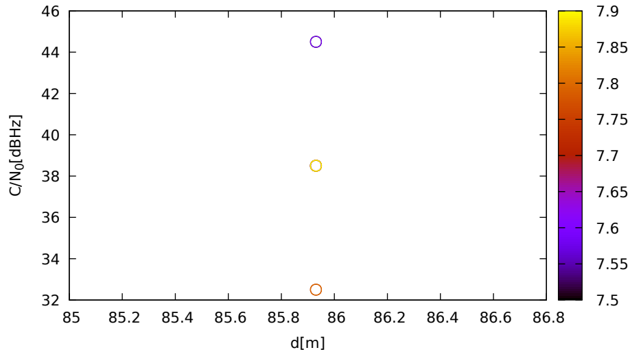
C/N 0 vs distance (LeicaGS15 at C 3 for G31 at L2)
