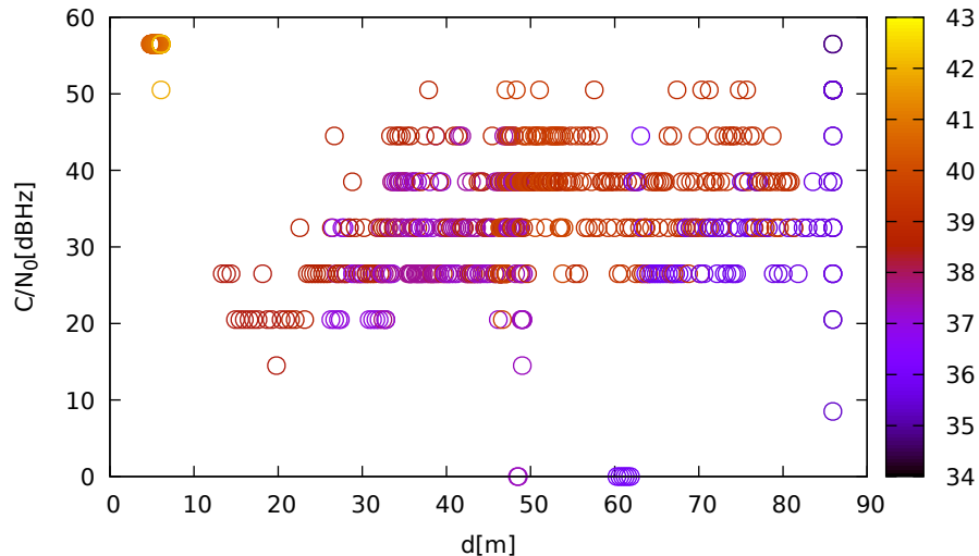
C/N 0 vs distance (LeicaGS15 at C 3 for G32 at L2)
