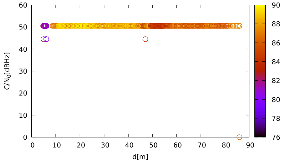
C/N 0 vs distance (LeicaGS15 at C 3 for R07 at L2)
