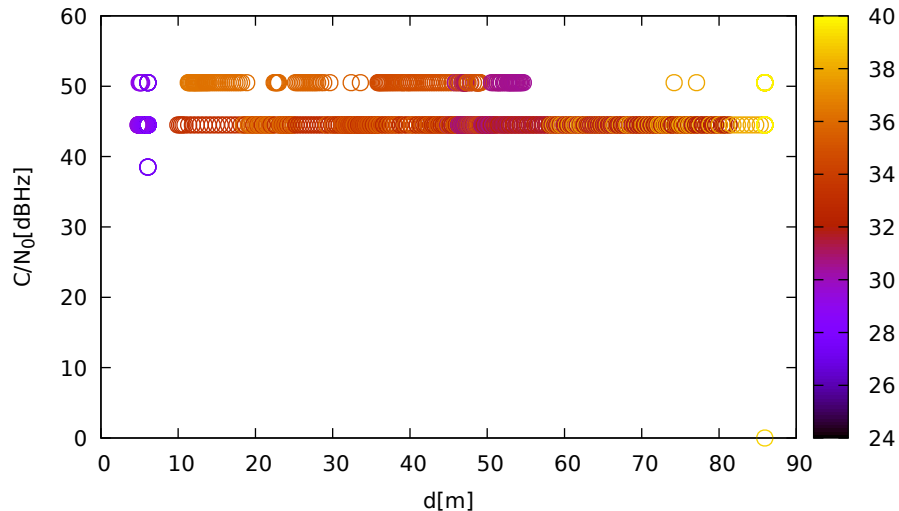
C/N 0 vs distance (LeicaGS15 at C 3 for R08 at L2)
