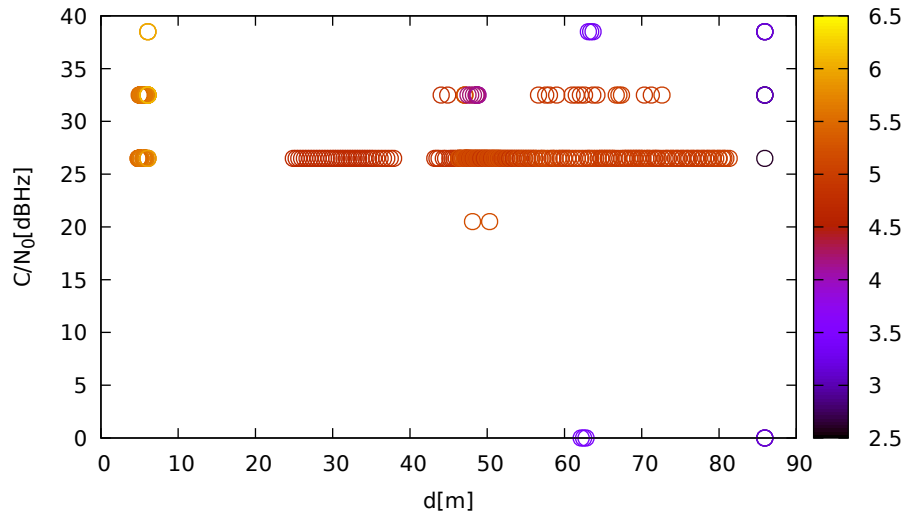
C/N 0 vs distance (LeicaGS15 at C 3 for R14 at L2)
