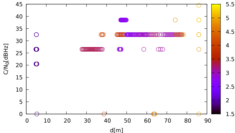
C/N 0 vs distance (LeicaGS15 at C 3 for R15 at L2)
