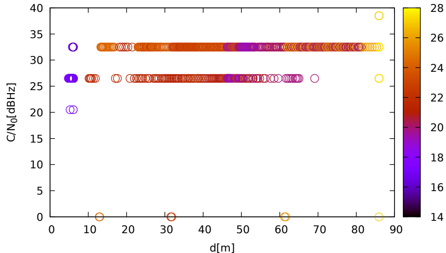
C/N 0 vs distance (LeicaGS15 at C 3 for R23 at L2)
