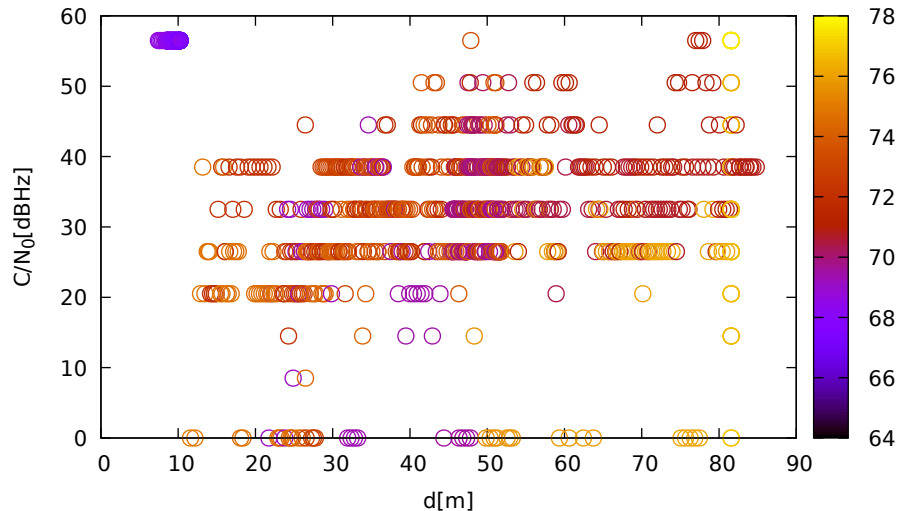
C/N 0 vs distance (LeicaGS18 at C 3 for G01 at L2)
