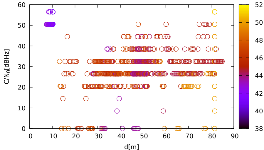
C/N 0 vs distance (LeicaGS18 at C 3 for G03 at L2)
