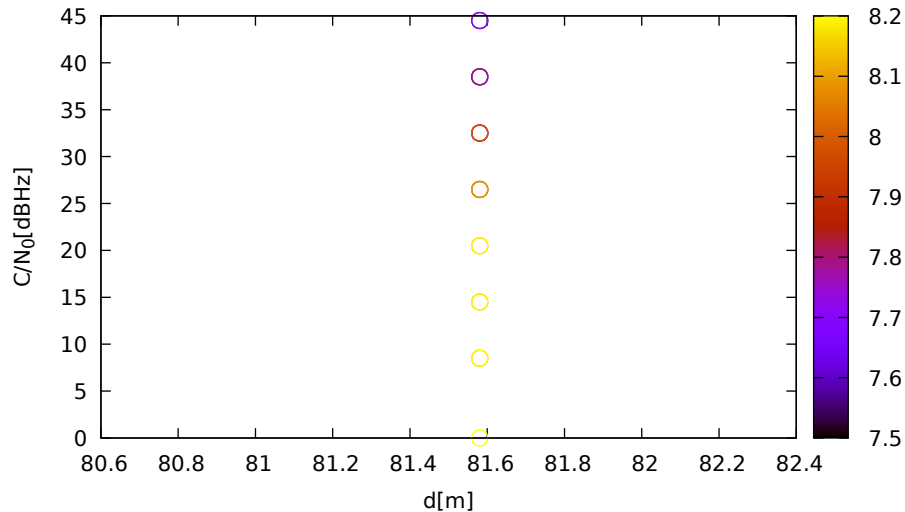
C/N 0 vs distance (LeicaGS18 at C 3 for G04 at L2)
