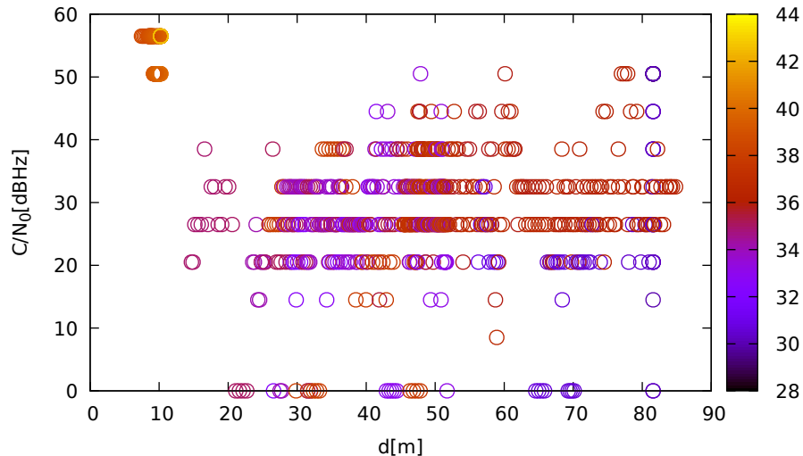
C/N 0 vs distance (LeicaGS18 at C 3 for G08 at L2)
