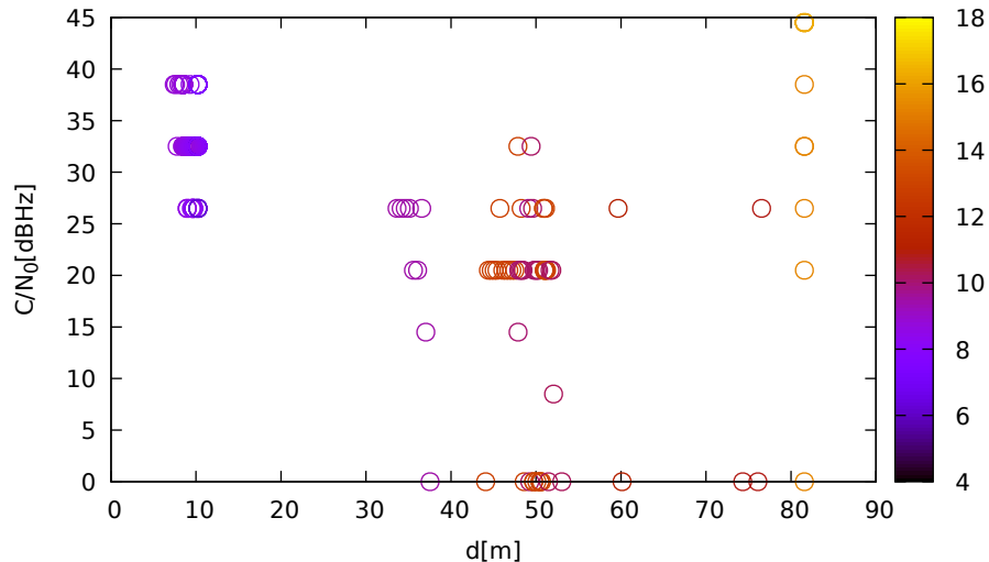
C/N 0 vs distance (LeicaGS18 at C 3 for G17 at L2)
