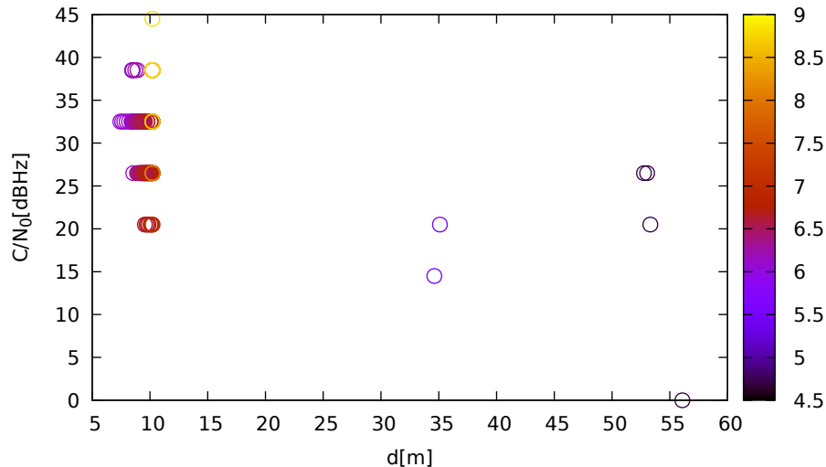
C/N 0 vs distance (LeicaGS18 at C 3 for G21 at L2)
