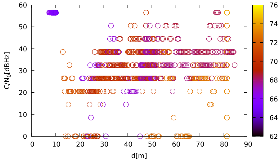
C/N 0 vs distance (LeicaGS18 at C 3 for G22 at L2)
