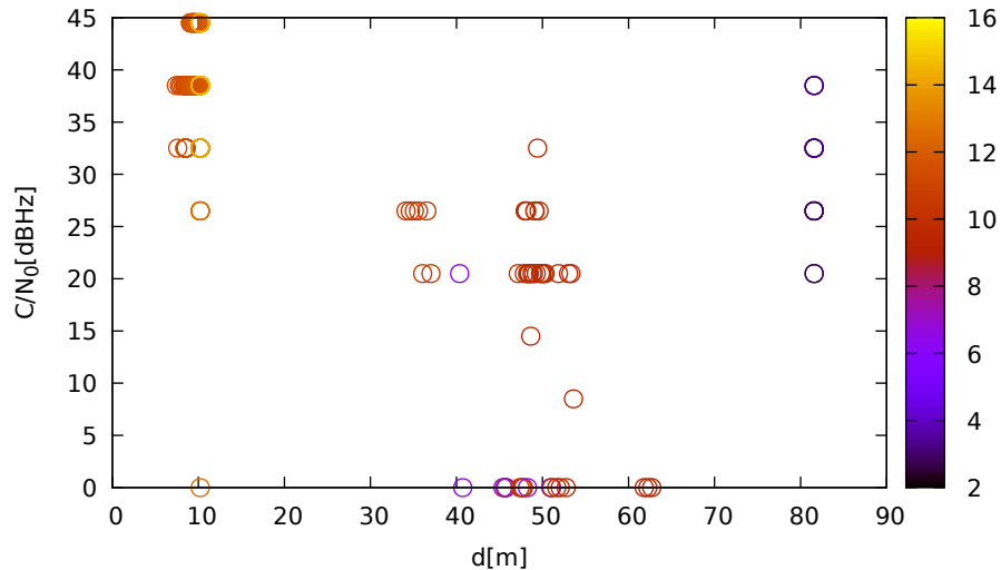
C/N 0 vs distance (LeicaGS18 at C 3 for G27 at L2)
