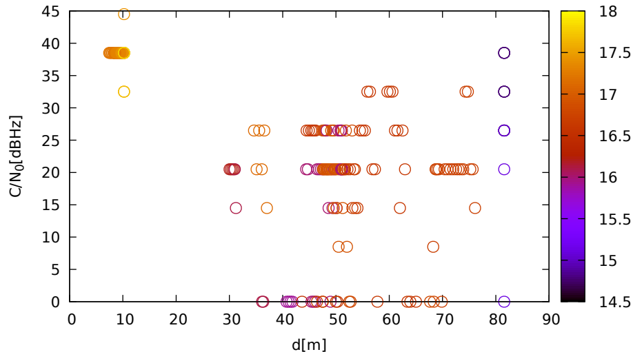
C/N 0 vs distance (LeicaGS18 at C 3 for G28 at L2)
