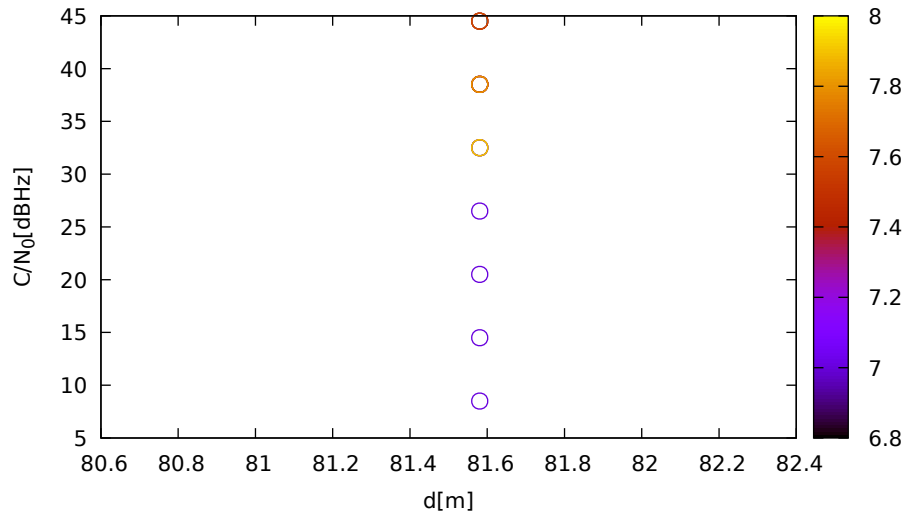
C/N 0 vs distance (LeicaGS18 at C 3 for G31 at L2)
