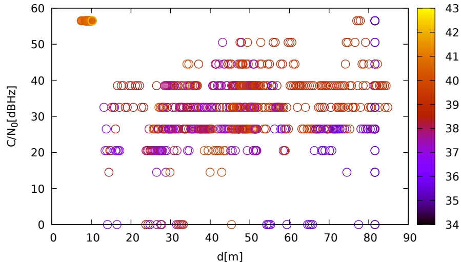
C/N 0 vs distance (LeicaGS18 at C 3 for G32 at L2)
