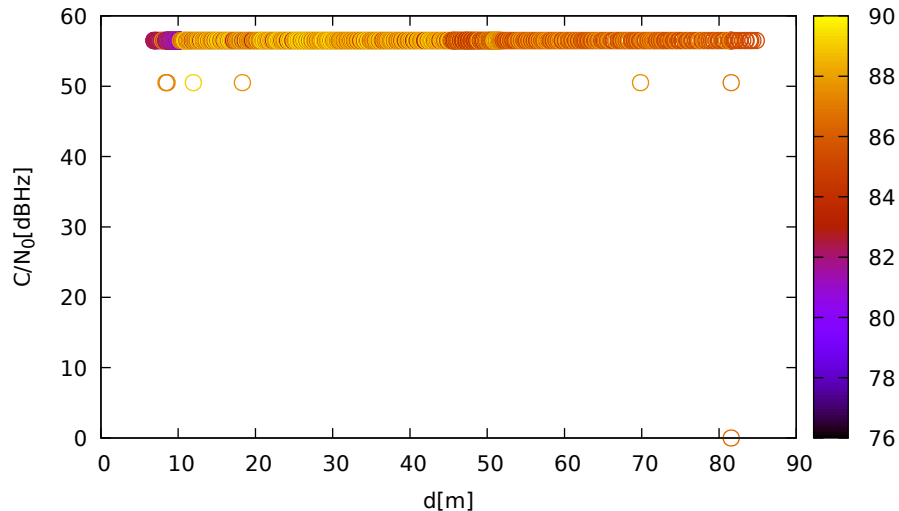
C/N 0 vs distance (LeicaGS18 at C 3 for R07 at L2)
