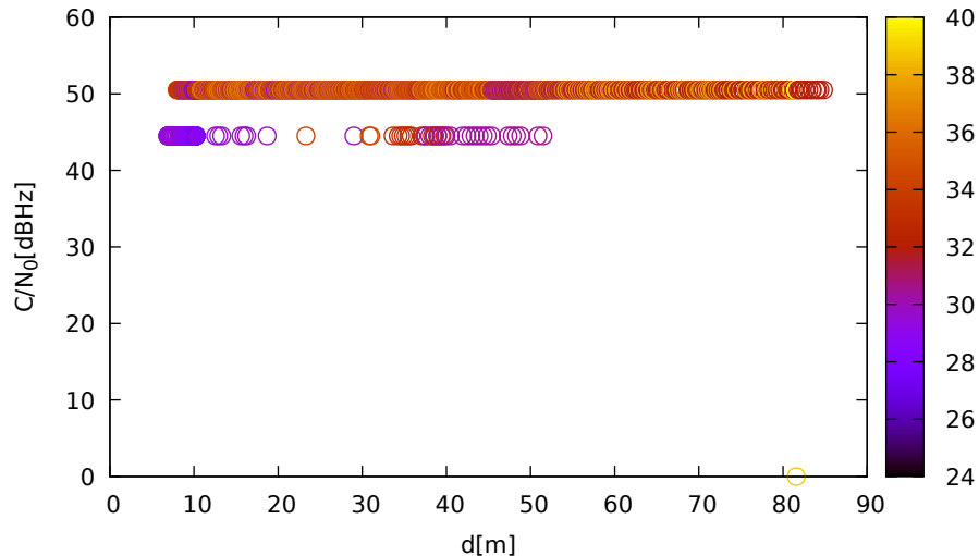
C/N 0 vs distance (LeicaGS18 at C 3 for R08 at L2)
