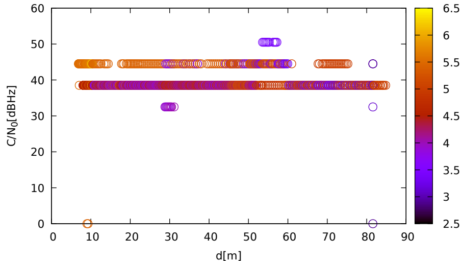
C/N 0 vs distance (LeicaGS18 at C 3 for R14 at L2)
