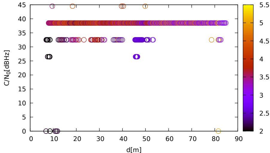
C/N 0 vs distance (LeicaGS18 at C 3 for R15 at L2)
