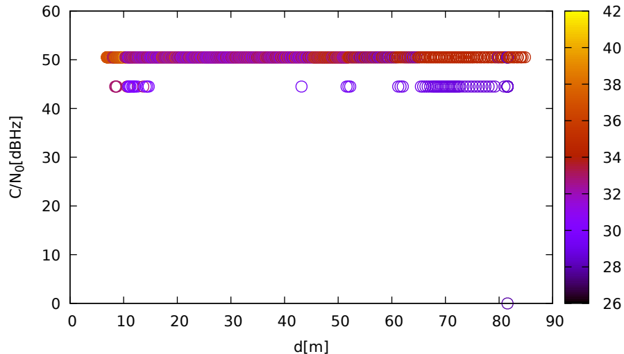
C/N 0 vs distance (LeicaGS18 at C 3 for R21 at L2)
