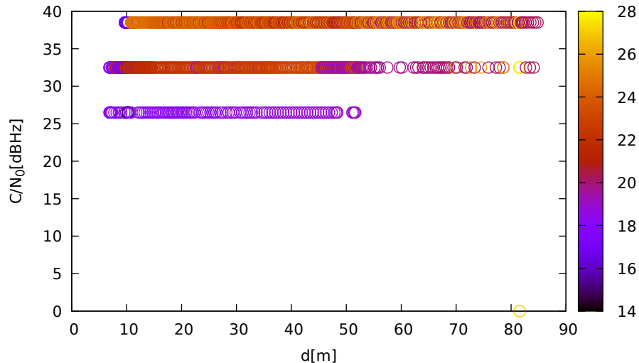
C/N 0 vs distance (LeicaGS18 at C 3 for R23 at L2)
