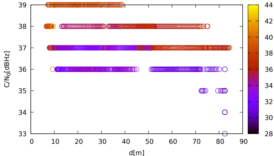
C/N 0 vs distance (ublox9 at C 3 for G08 at L2)
