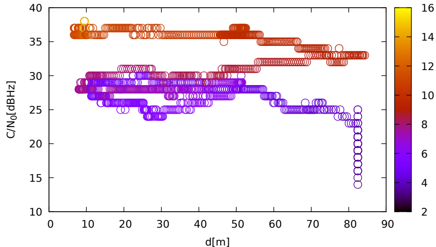
C/N 0 vs distance (ublox9 at C 3 for G27 at L2)
