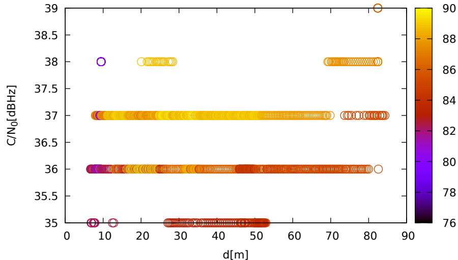
C/N 0 vs distance (ublox9 at C 3 for R07 at L2)
