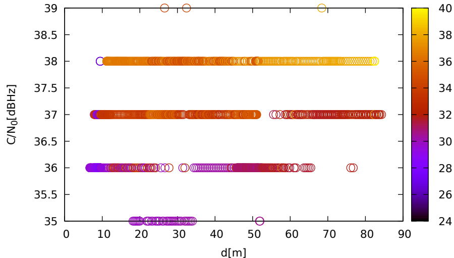
C/N 0 vs distance (ublox9 at C 3 for R08 at L2)
